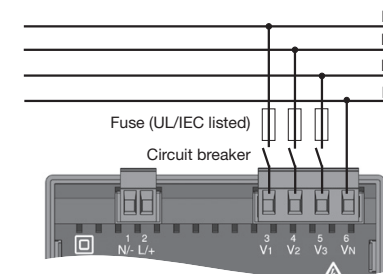
Voltage measurement connection variant 3p 4w (Addr. 509 = 0, default setting)
