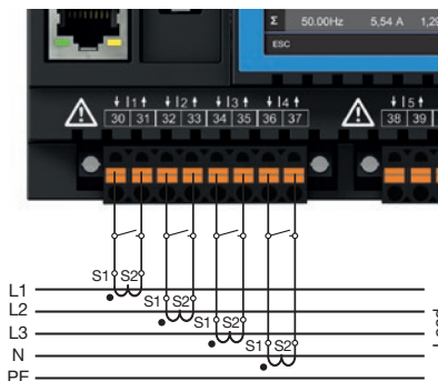
Fig. Connection example for "current measurement".
