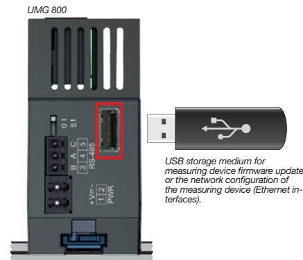
Fig. Measuring device - view from below
