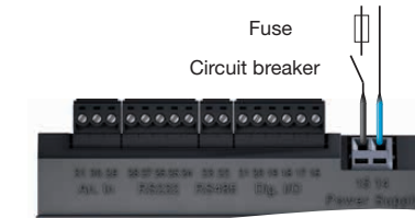
Fig. Connecting U h supply voltage.
